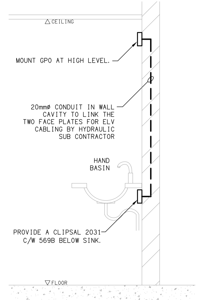
DETAIL AUTO TAP CONNECTION NOT TO SCALE
